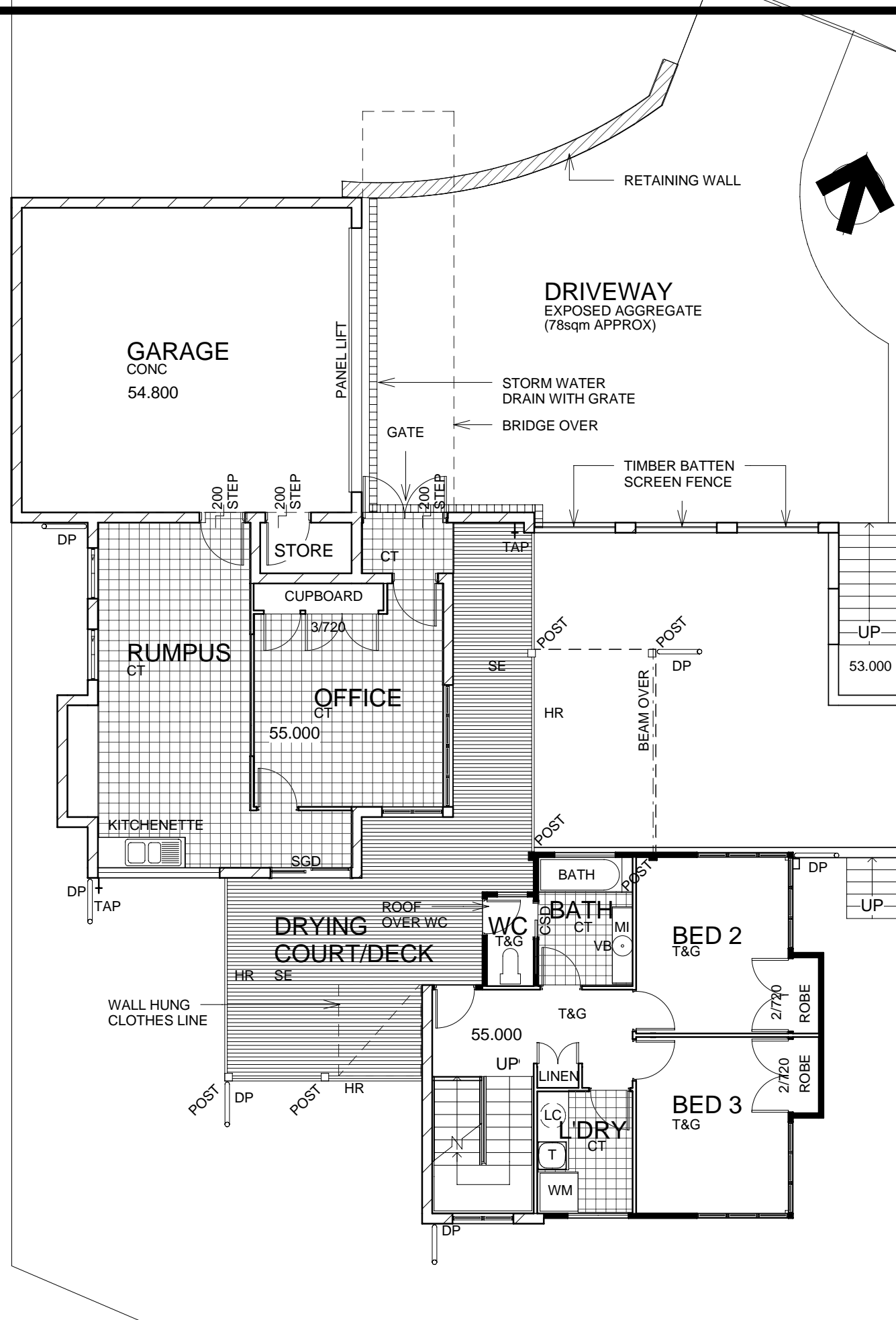
1 WD07 1 : 100 GROUND F.L. PLAN
